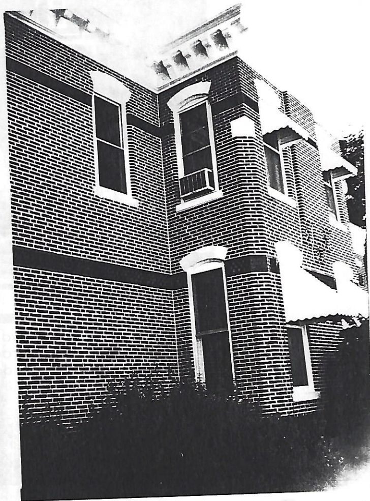
Detail of the West facade with wood cornice, brackets and carvings at the roofline, the decorative brick belt-courses, and segmental brick arch windows with stone sills
