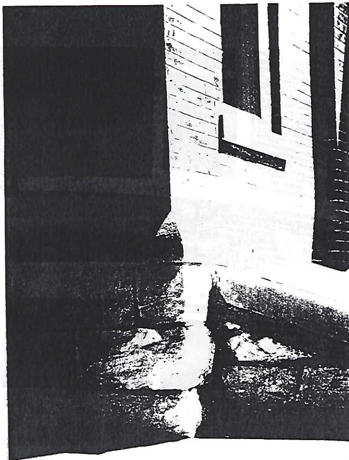
Detail of the limestone foundation walls, smooth-cut stone water table and brick exterior walls
