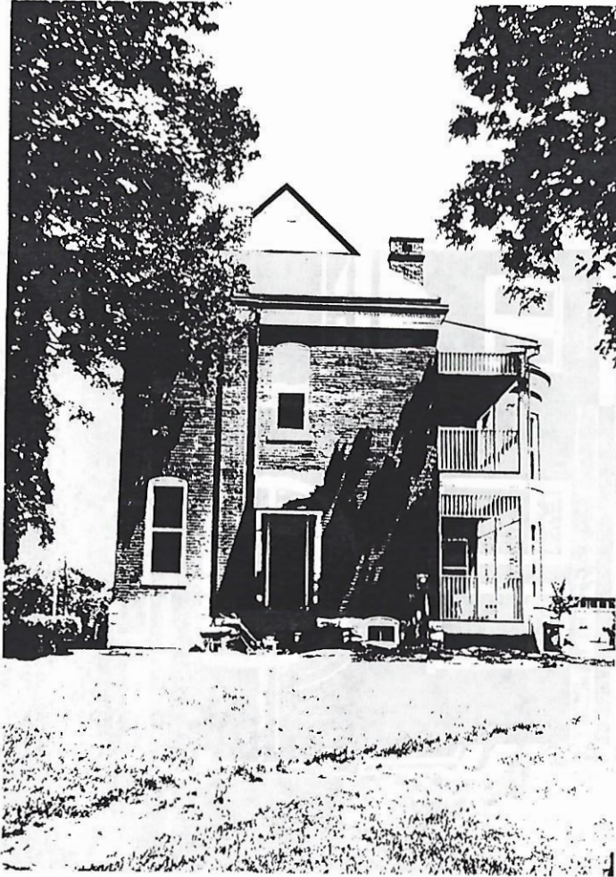
South Facade-Shows chimney; roof shape; rear entry; window configuration; massing; materials.
